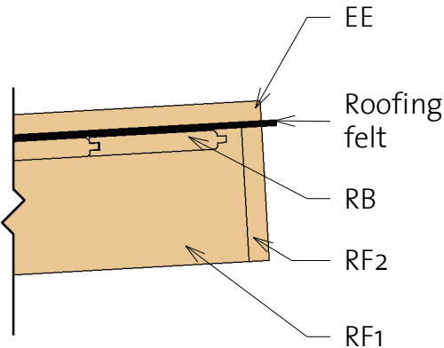
4 Roof Reinforcement
